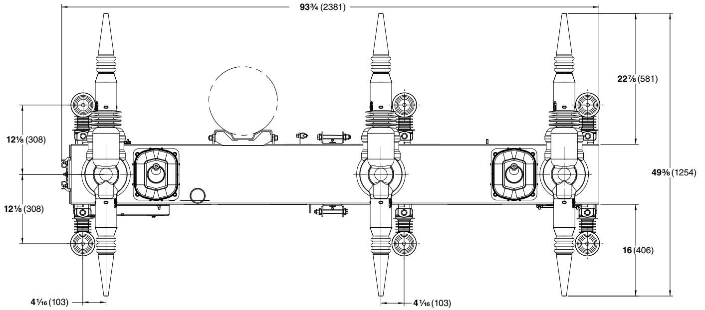
TOP VIEW
