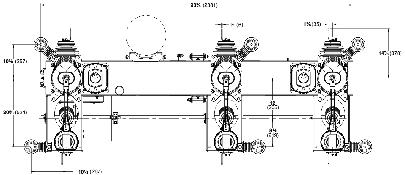
TOP VIEW
