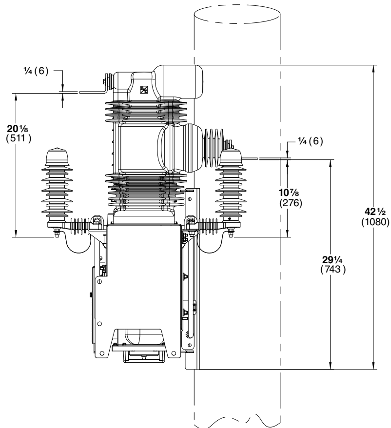
SIDE VIEW
