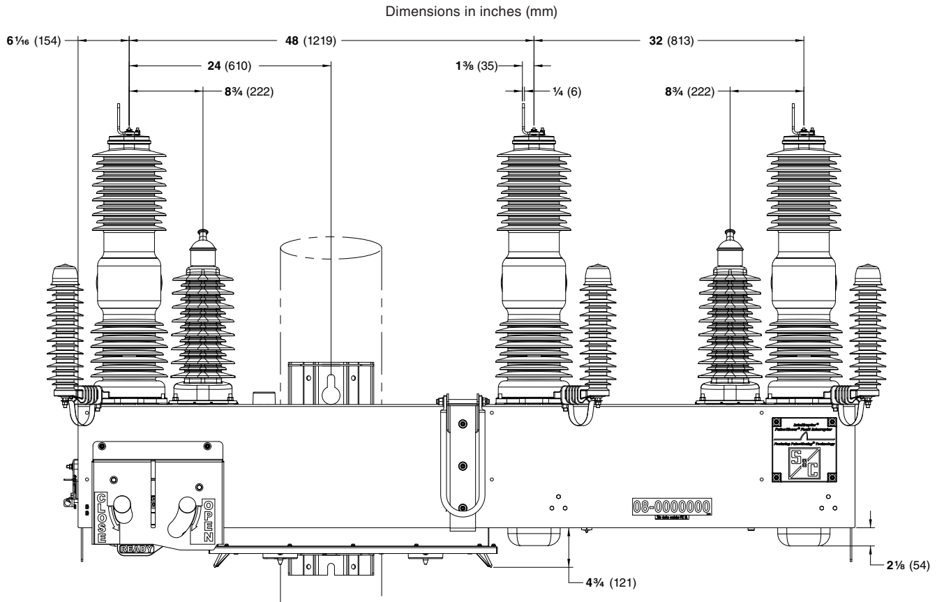
FRONT VIEW
