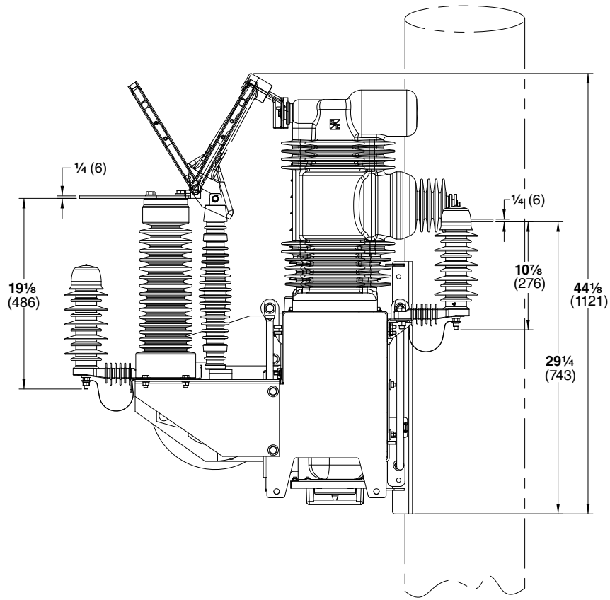
SIDE VIEW
